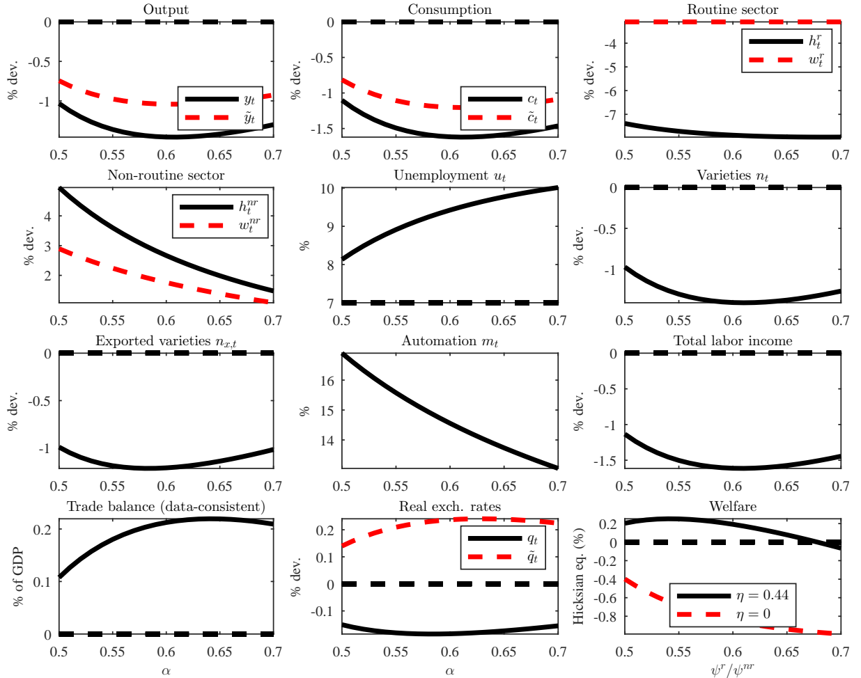
Figure 4: Effects after 100 quarters, varying the output elasticity to non-routine labor ( \alpha ).
