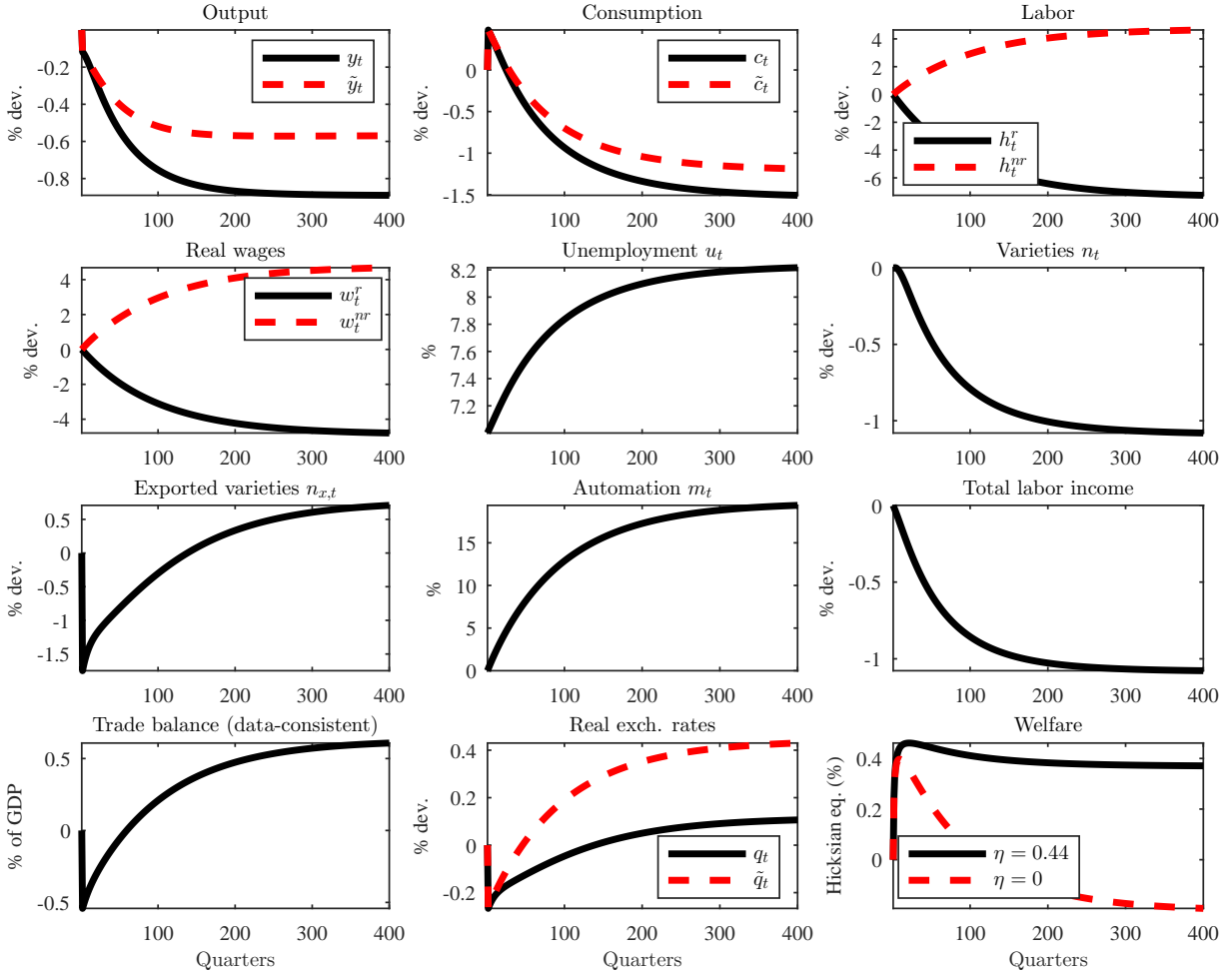
Figure 5: The effects of a permanent automation shock with GHH preferences.
