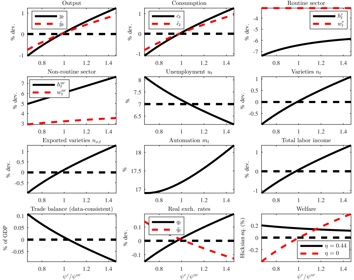
Figure 3: Effects after 100 quarters, varying the relative elasticity of non-routine labor supply.
