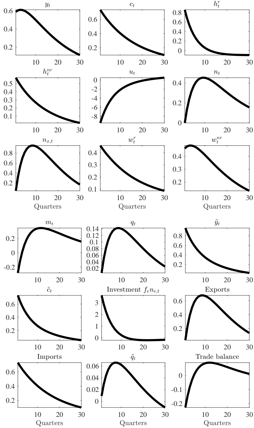
Figure 1: IRFs to a 1 sd positive labor productivity shock.
