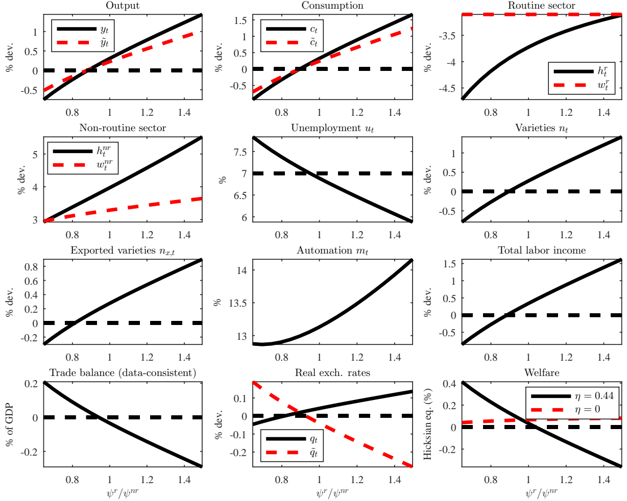
Figure 8: Effects after 100 quarters, varying the relative elasticity of non-routine labor supply with GHH preferences
