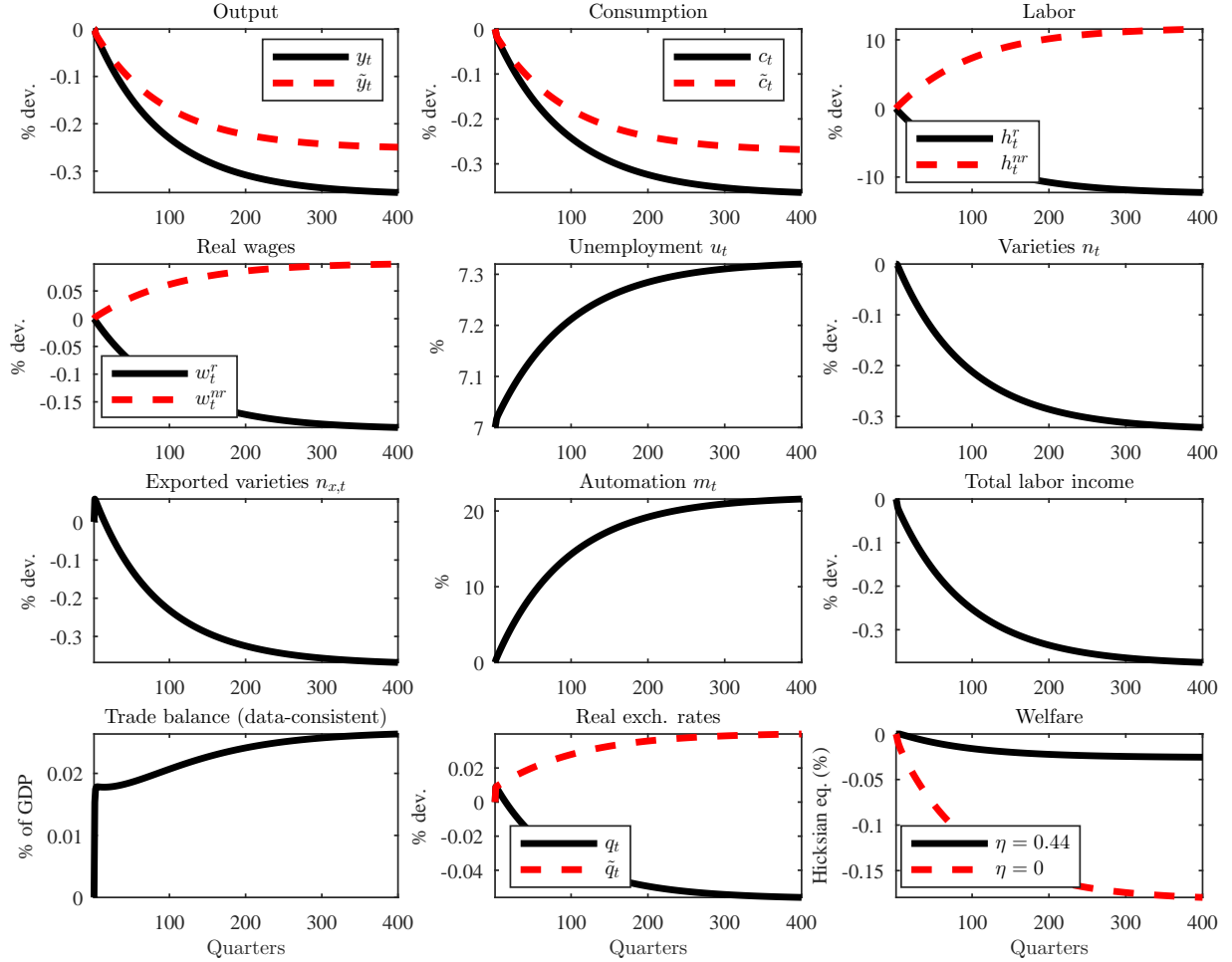
Figure 6: The effects of a permanent automation shock with quasi-indivisible labor
