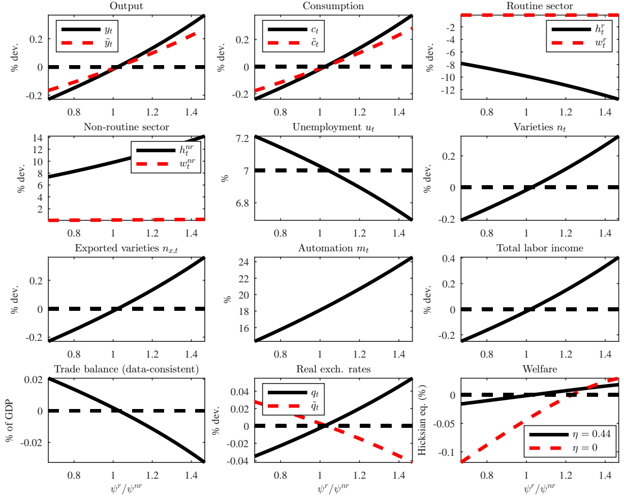
Figure 9: Effects after 100 quarters, varying the relative elasticity of non-routine labor supply with quasi-indivisible labor
